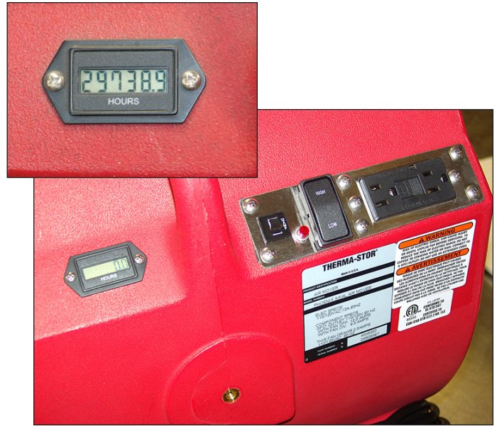
Innovative control panel includes power-on light, run-time hour meter, GFCI outlet and more.
