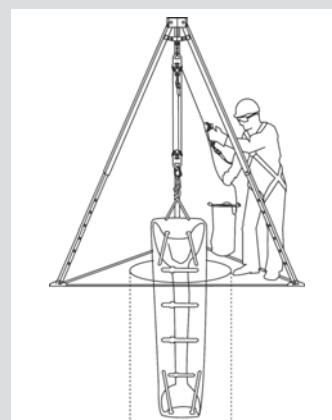
The SuretyMan Rescue Utility System can be used in conjunction with the Sure-Strong Tripod and Sked Rescue system
